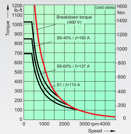
1PH7226-2.B.-..... max. breakdown torque: 1661 lb-ft/2252 Nm
