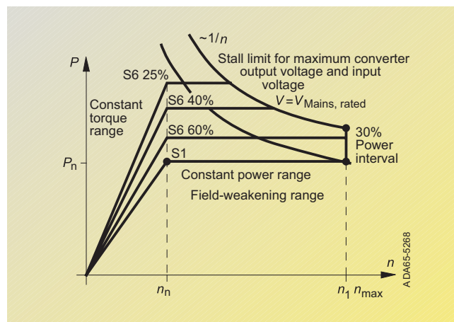
Fig. 3/8 Power-speed characteristic
